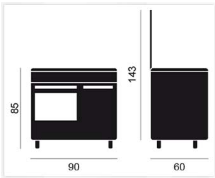
Porta-Bombonas CB96PBB
